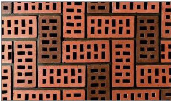
Product No. P718 Zig-Zag Brick Size (Millimeter) 220 x 104 x 68 L W T
